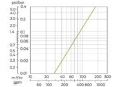
Head Loss Graph (in clean water)
