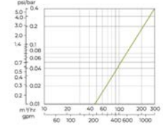
Head Loss Graph (in clean water)
